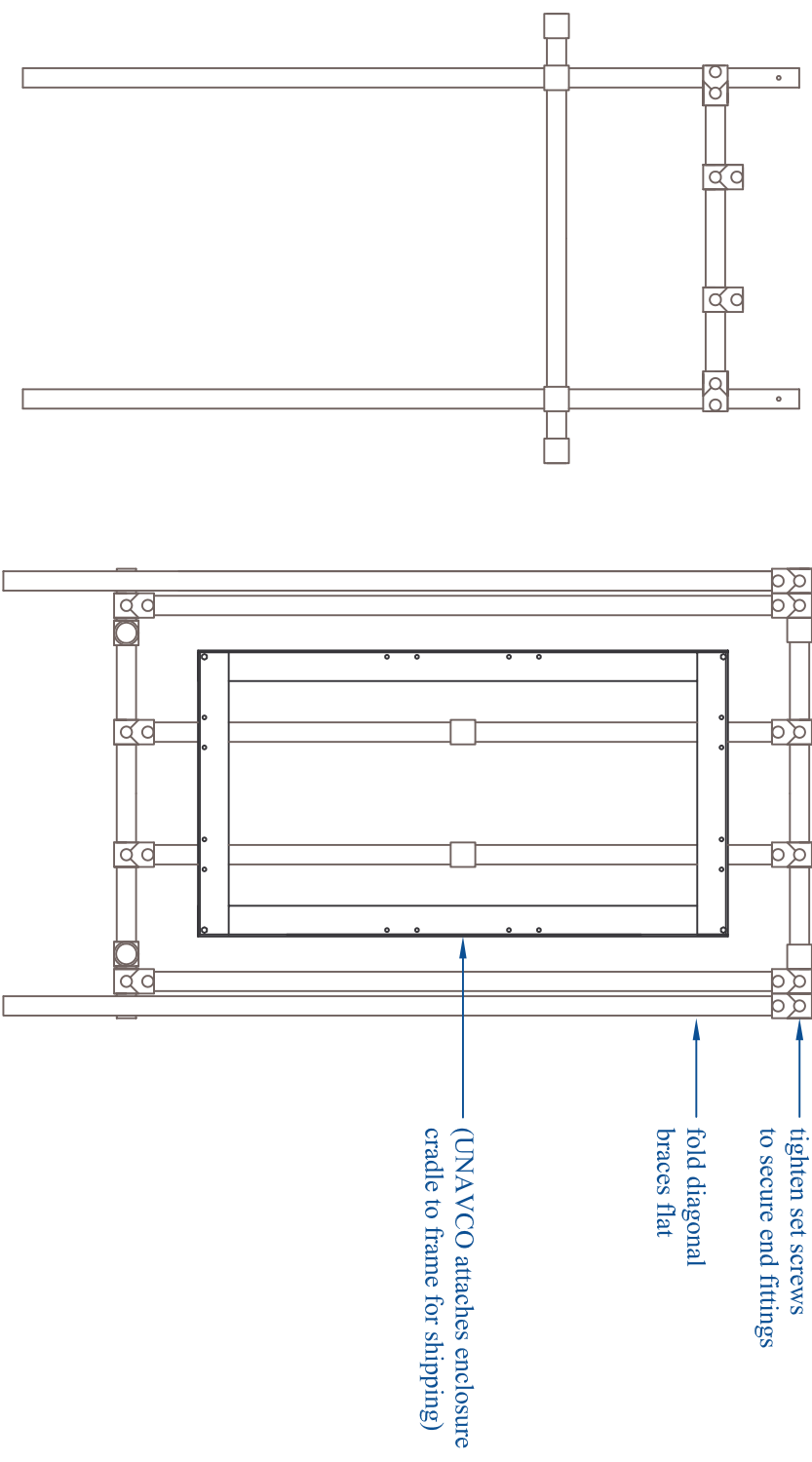
Disassembly of Frame for Shipping
