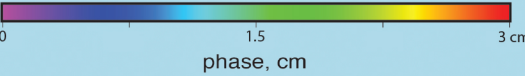
Sentinel-1A Path 128 Tops Mode 2015/05/06 - 2015/06/23
